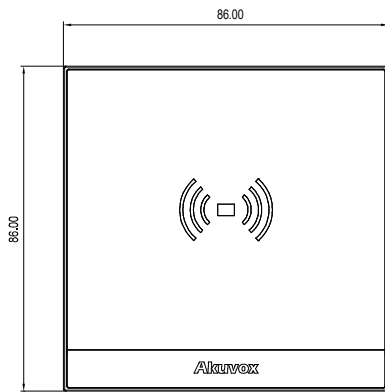
1 FRONT VIEW
