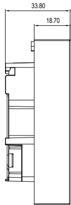
2 RIGHT VIEW
